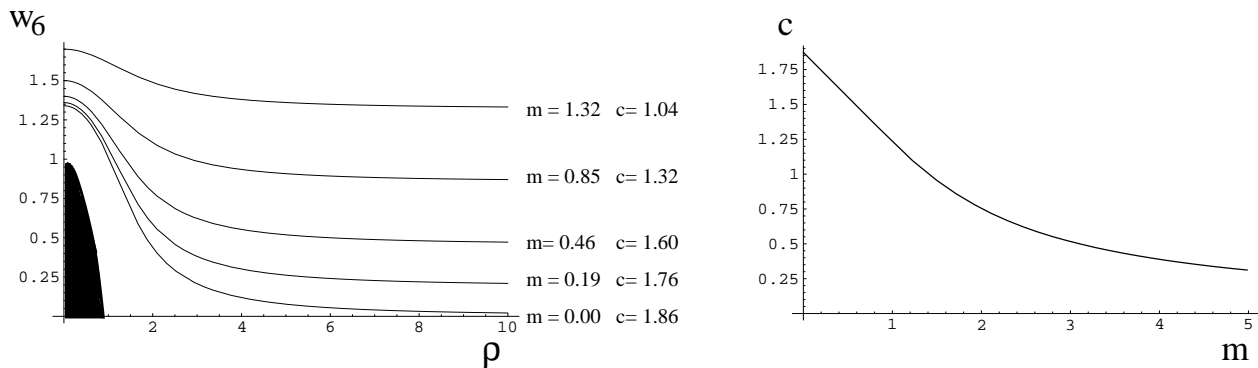
Figure 5.4: Numerical solutions for D7 embeddings in the Constable-Myers geometry with b = 1 . The shaded area corresponds to the singularity in the metric. Also plotted is the value of the quark condensate vs the mass extracted asymptotically from those flows.
