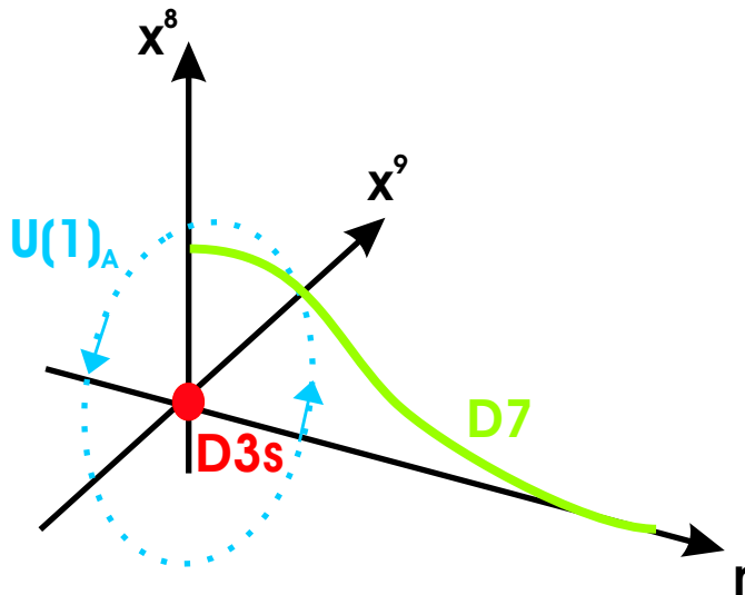
Figure 5.1: Geometric chiral symmetry breaking in a D3-D7 system.
