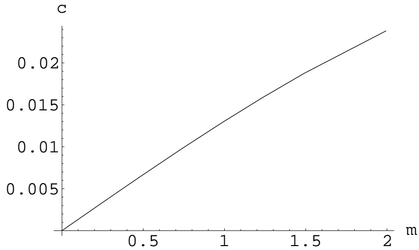
Figure 5.3: Apparent values of the quark mass and condensate extracted asymptotically from the flows in Figure 5.2.
